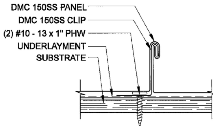
(Perimeter and Corner Condition – Option 2 Seam Detail)
