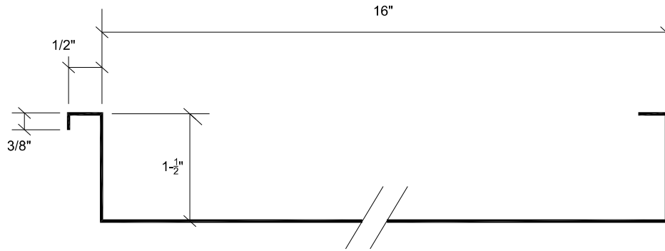
DCM 150 SS – 24GA. STEEL PANEL
