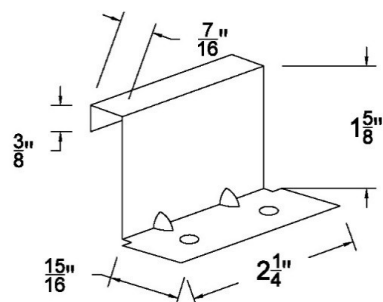
24 GA, DMC 150SS FIXED CLIP
