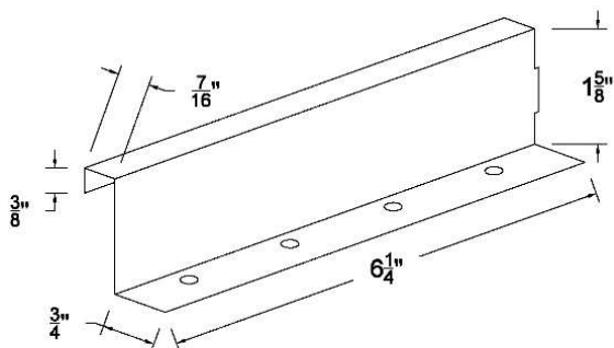
22 GA, DMC 150SS FIXED CLIP
