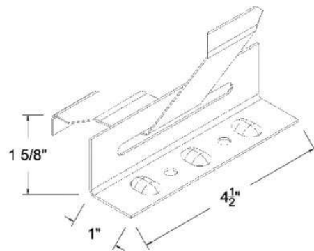
DMC 150SS BUTTERFLY CLIP
