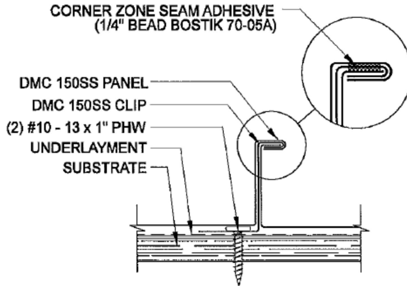
(Perimeter and Corner Condition – Option 1 Seam Detail)
